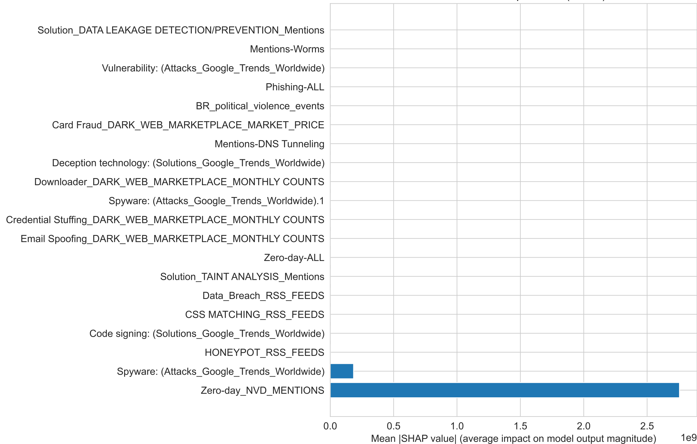
Global Feature Importance (SHAP)
